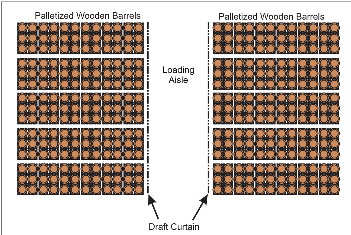
Fig. 2.4.8.3.A. Loading aisle draft curtain arrangement (plan view)
