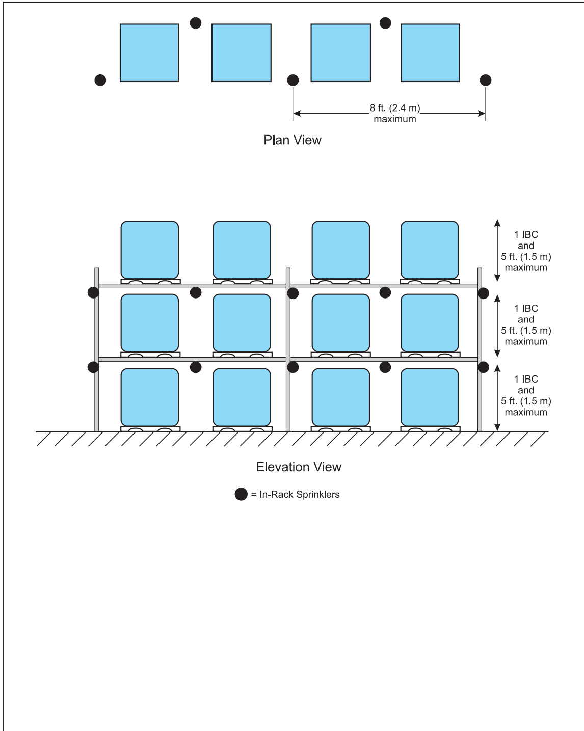
Fig. D.2.1.1. Single-row rack sprinkler layout: IBC protection scheme
