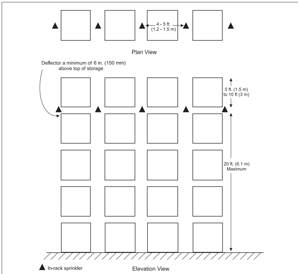
Fig. D.2.2.5.1. Single-row rack sprinkler layout: fire protection scheme E
