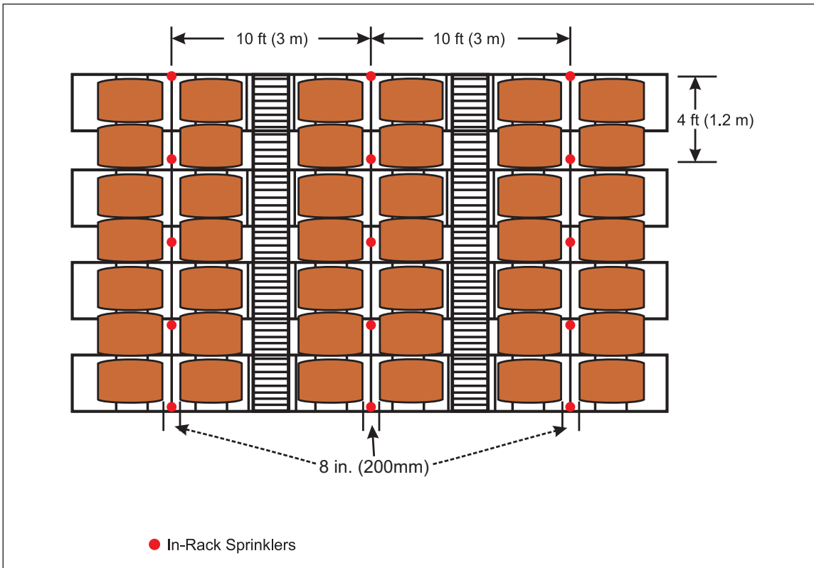
Fig. D.2.1.48. In-rack sprinkler layout for distilled spirits in wooden barrels (plan view)
