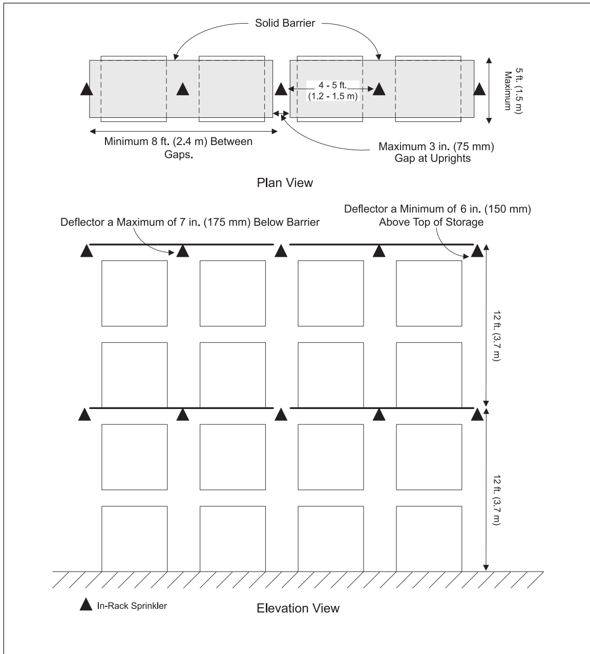
Fig. D.2.2.1.1. Single-row rack sprinkler layout: fire protection scheme A
