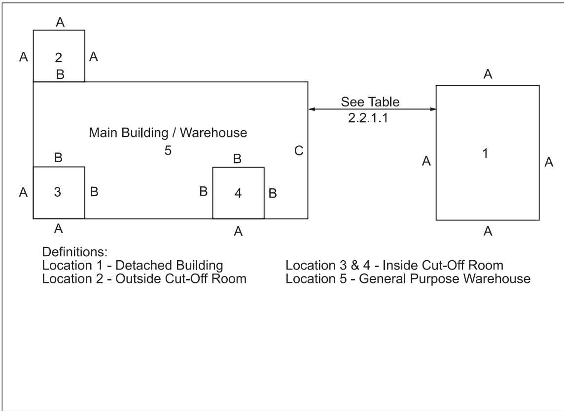
Fig. 2.2.1.1. Location and construction of ignitable liquid storage buildings and cutoff rooms
