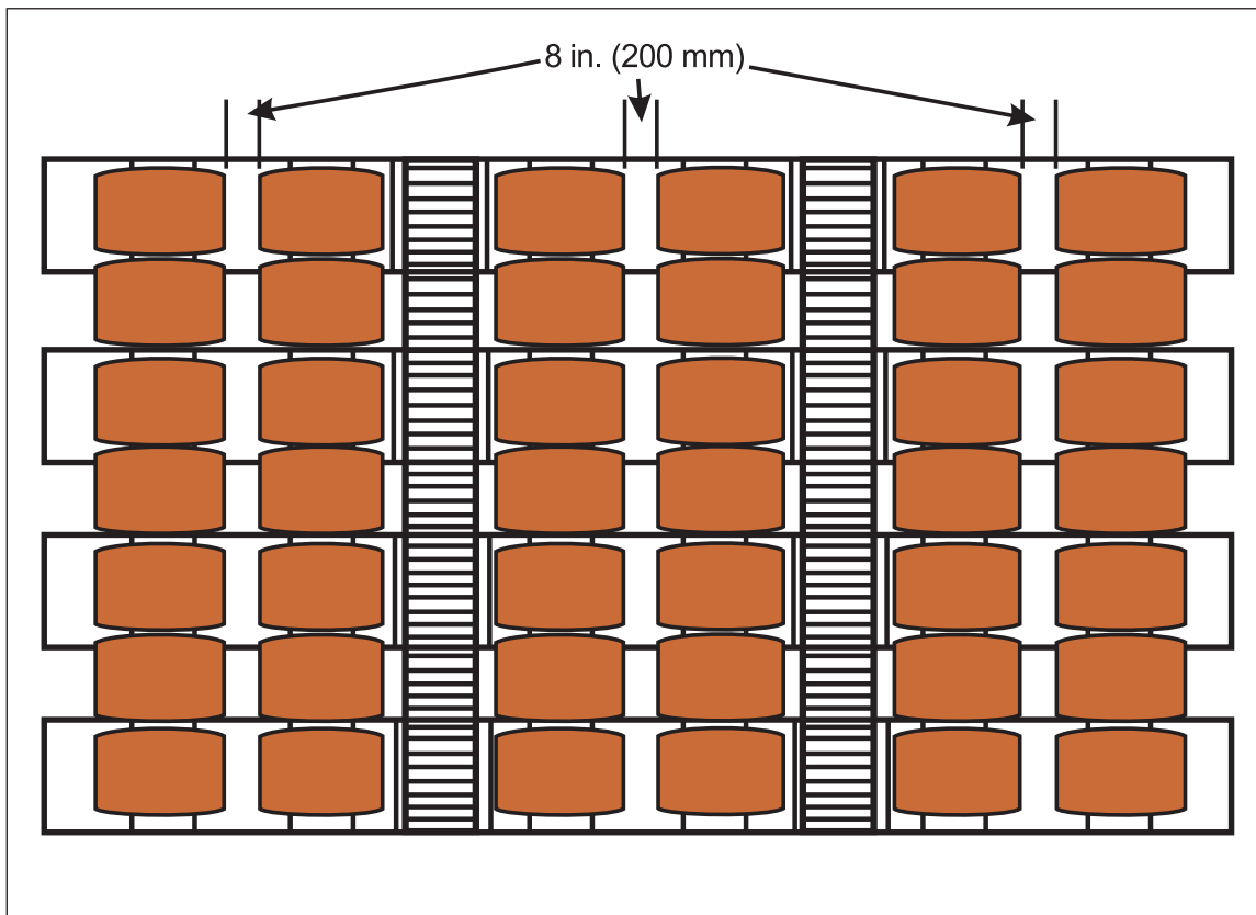
Fig. 2.4.9.1. Flue space and walkway layout for on-side barrel storage in racks (plan view)
