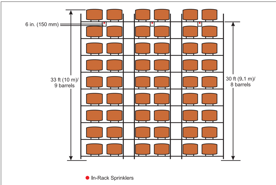
Fig. D.2.1.49. In-rack sprinkler layout for distilled spirits in wooden barrels (elevation view)
